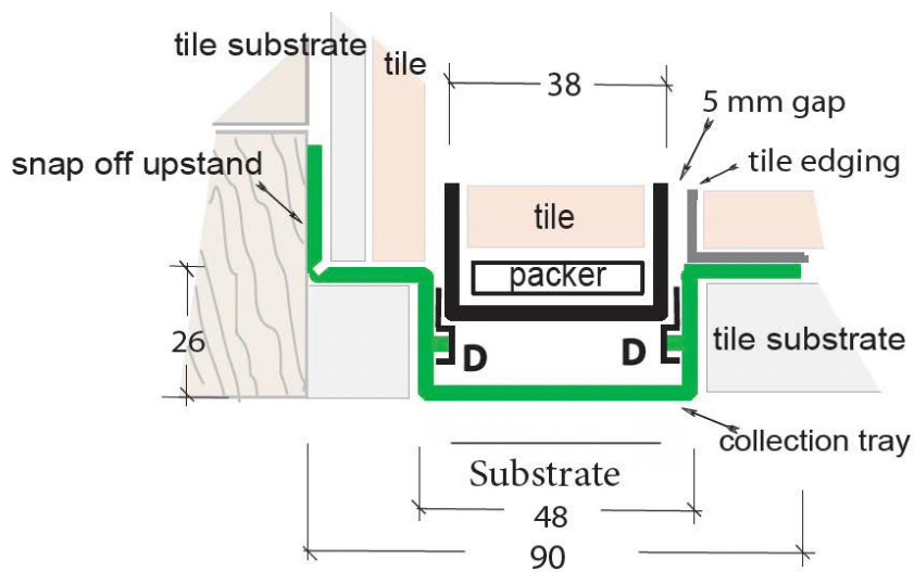
Cut away diagram
